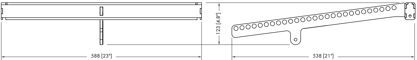
Z5394 Y Flying adapter dimensions in mm [inch]
